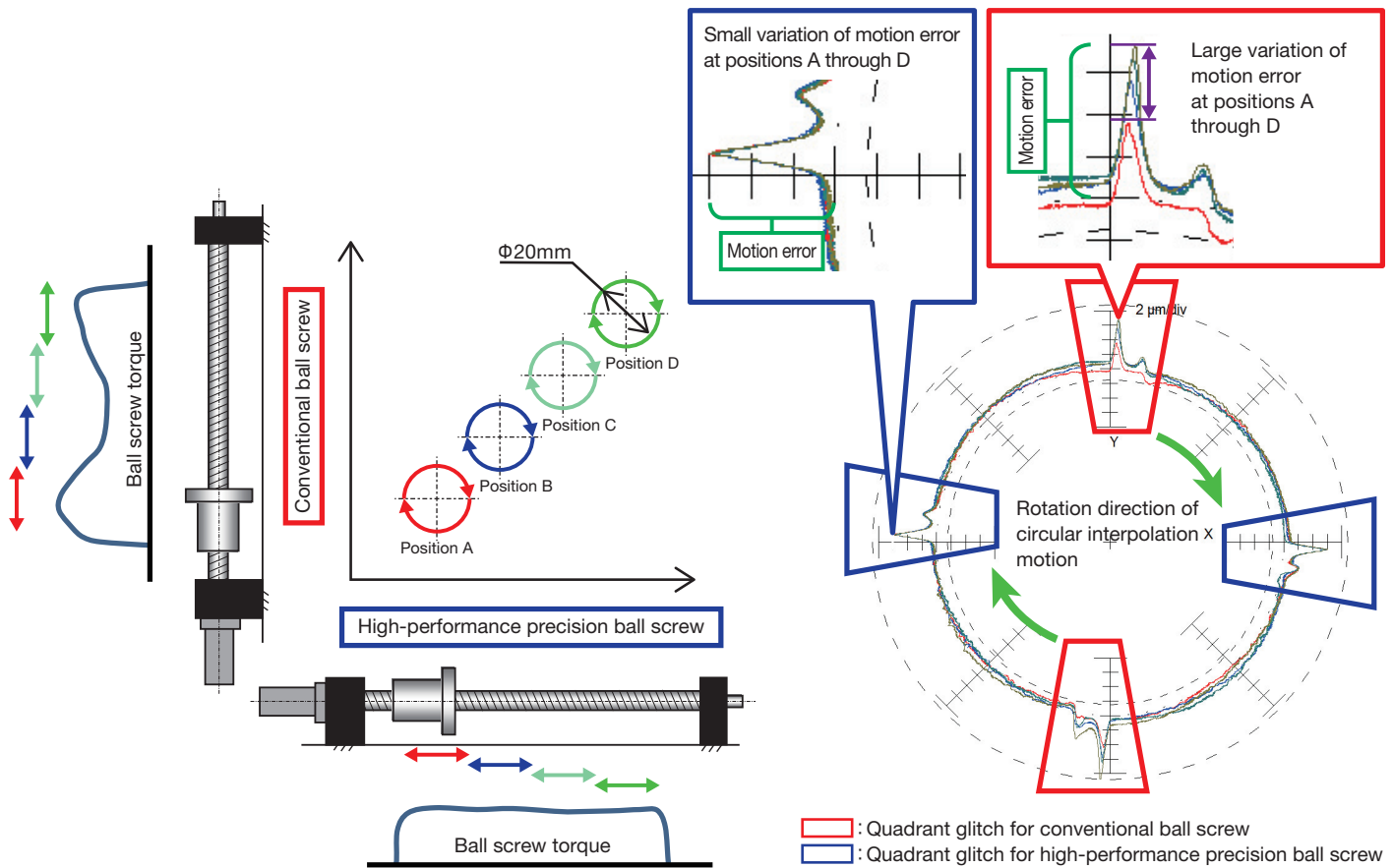
Figure 1 Position setting for orthogonal two-axis circular interpolation motion evaluation
